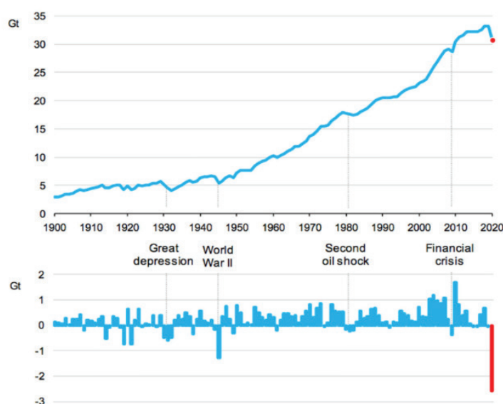
Figure 20. Global energy-related emissions (top) and annual change (bottom) in GtCO 2 , with projected 2020 levels highlighted in red
